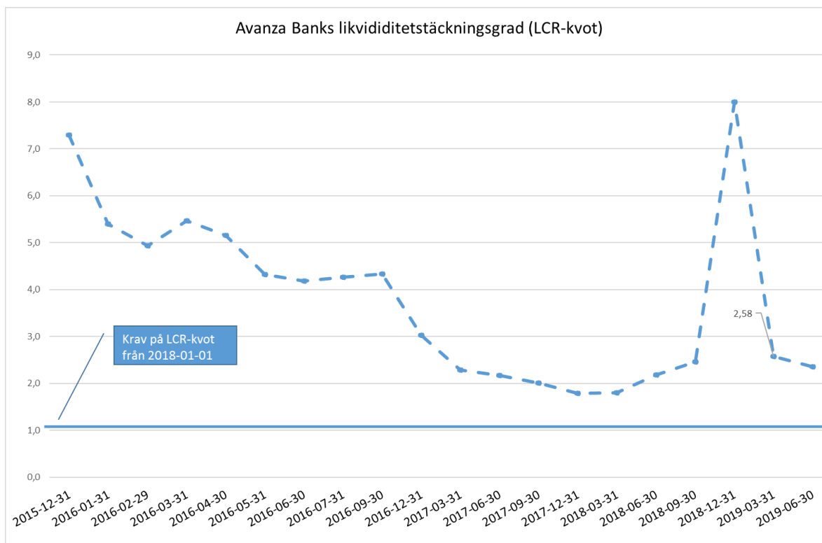
Diagram 2: Avanza Banks likvida situation.
